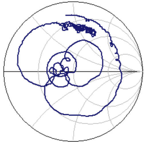
Smith Chart
