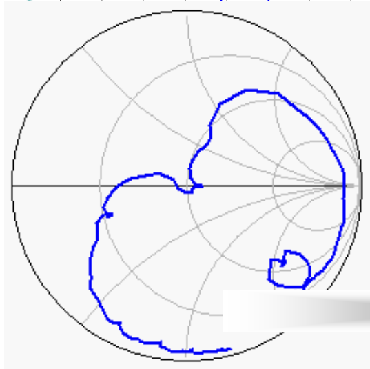
Return Loss
